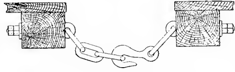
Fig. 5551. Cross Section of End-sills.
